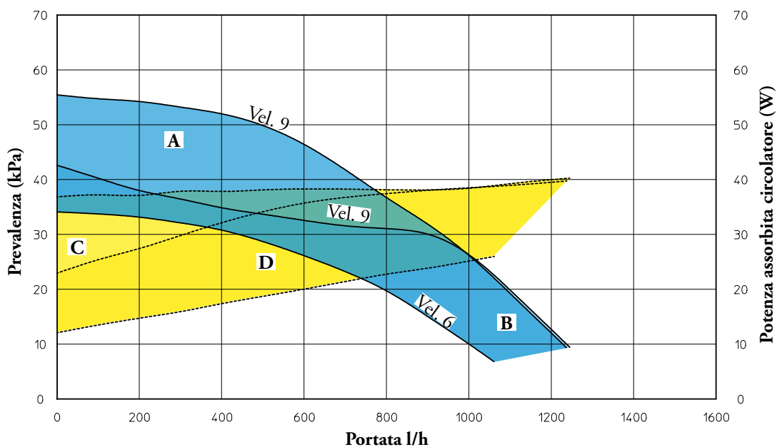
VICTRIX ZEUS 25 - GRUNDFOS UPM 3 15-60
